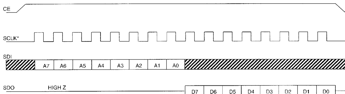
Figure 7. SPI SINGLE-BYTE READ
