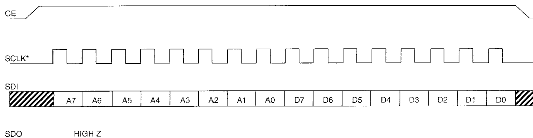
Figure 6. SPI SINGLE-BYTE WRITE
